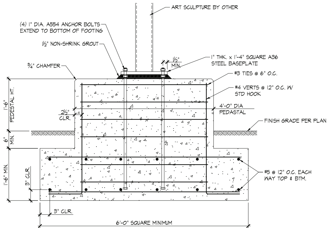
SECTION VIEW
