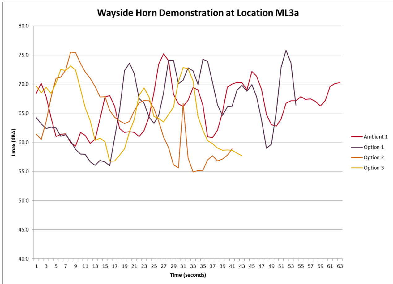
Figure 4-6. Wayside Horn Lmax at ML3a
