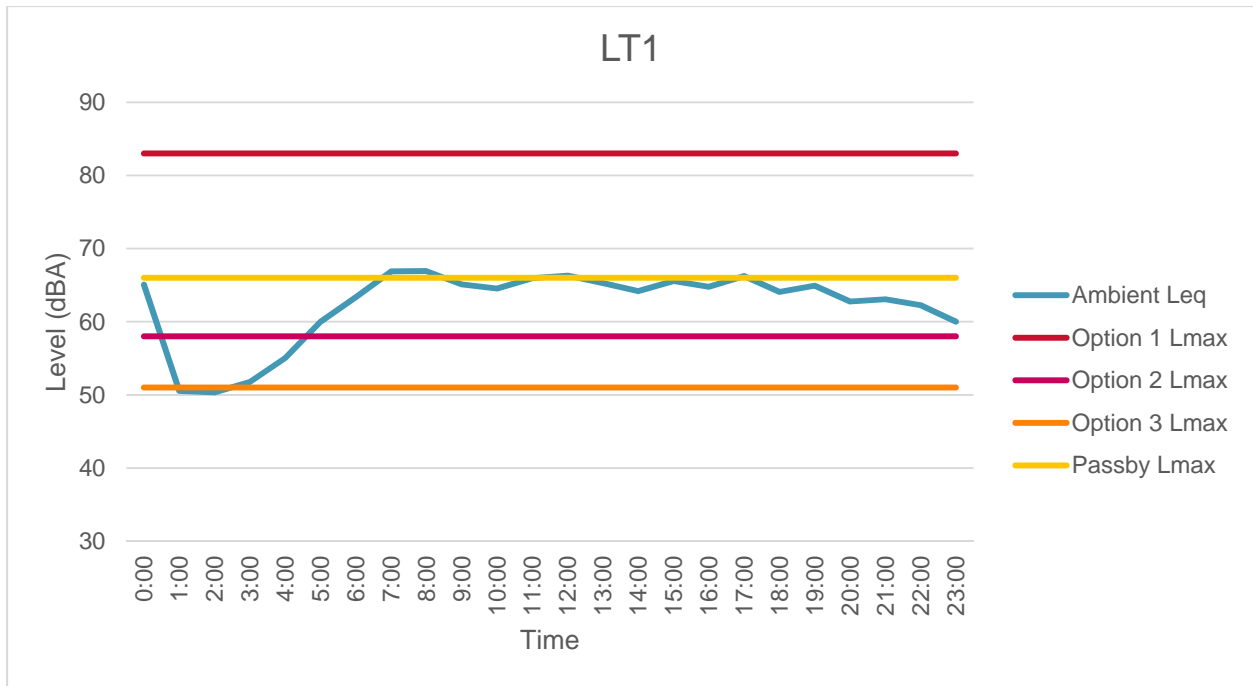
Figure 4-8. Comparison of Wayside Horns Lmax and Ambient Leq at LT1
