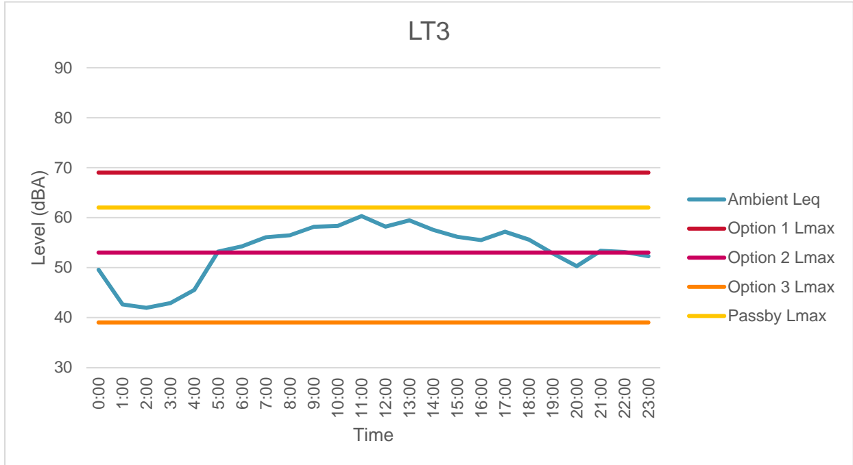
Figure 4-10. Comparison of Wayside Horns Lmax and Ambient Leq at LT3
