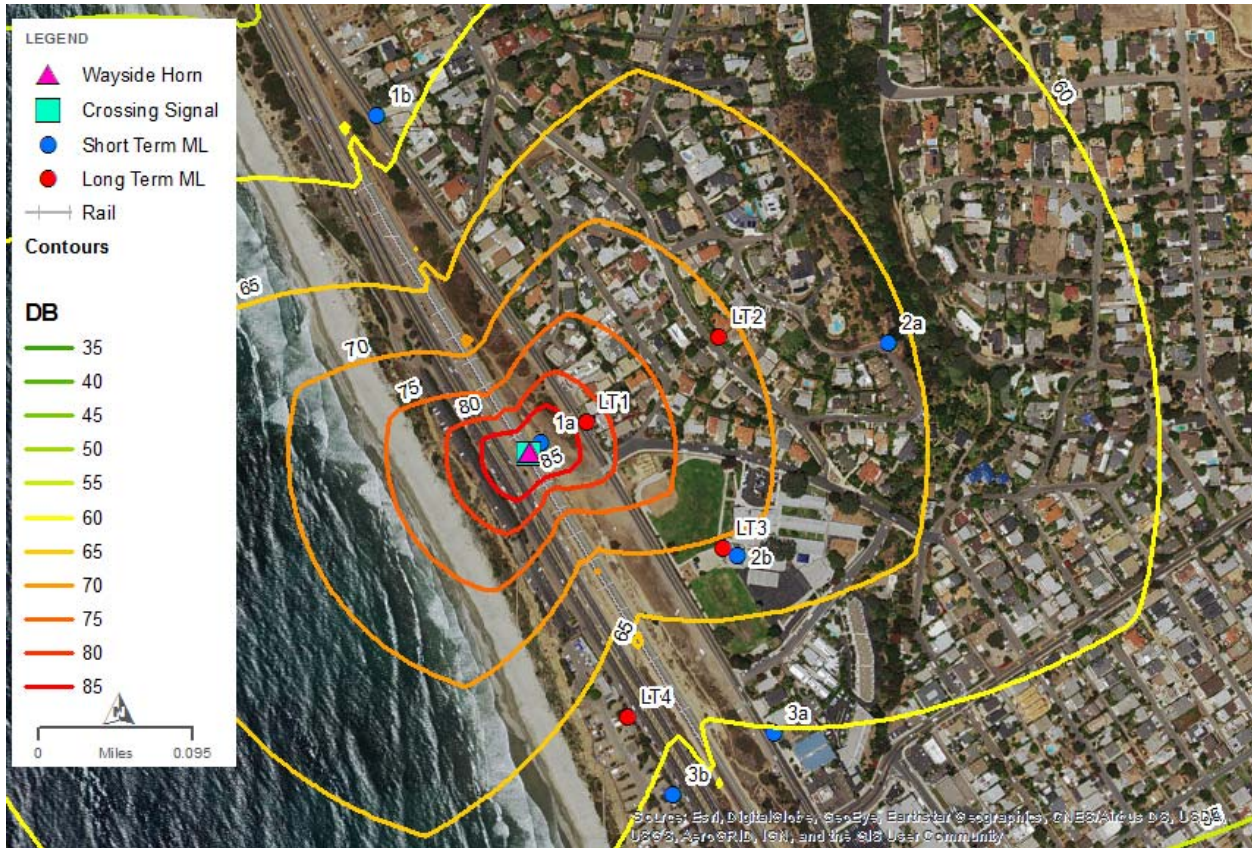
Figure 4-16. Option 1 Wayside Horn Noise Contours
