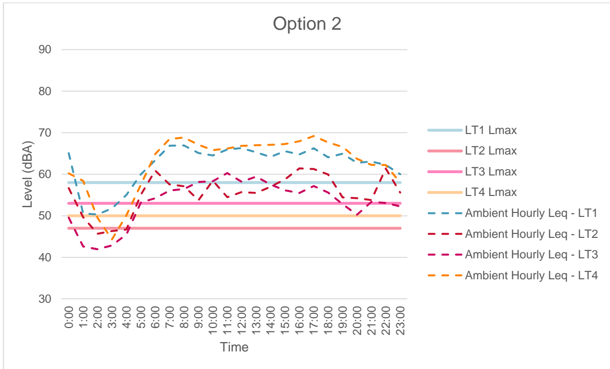
Figure 4-13. Option 2 Lmax vs. Leq at 24-hour Measurement Locations
