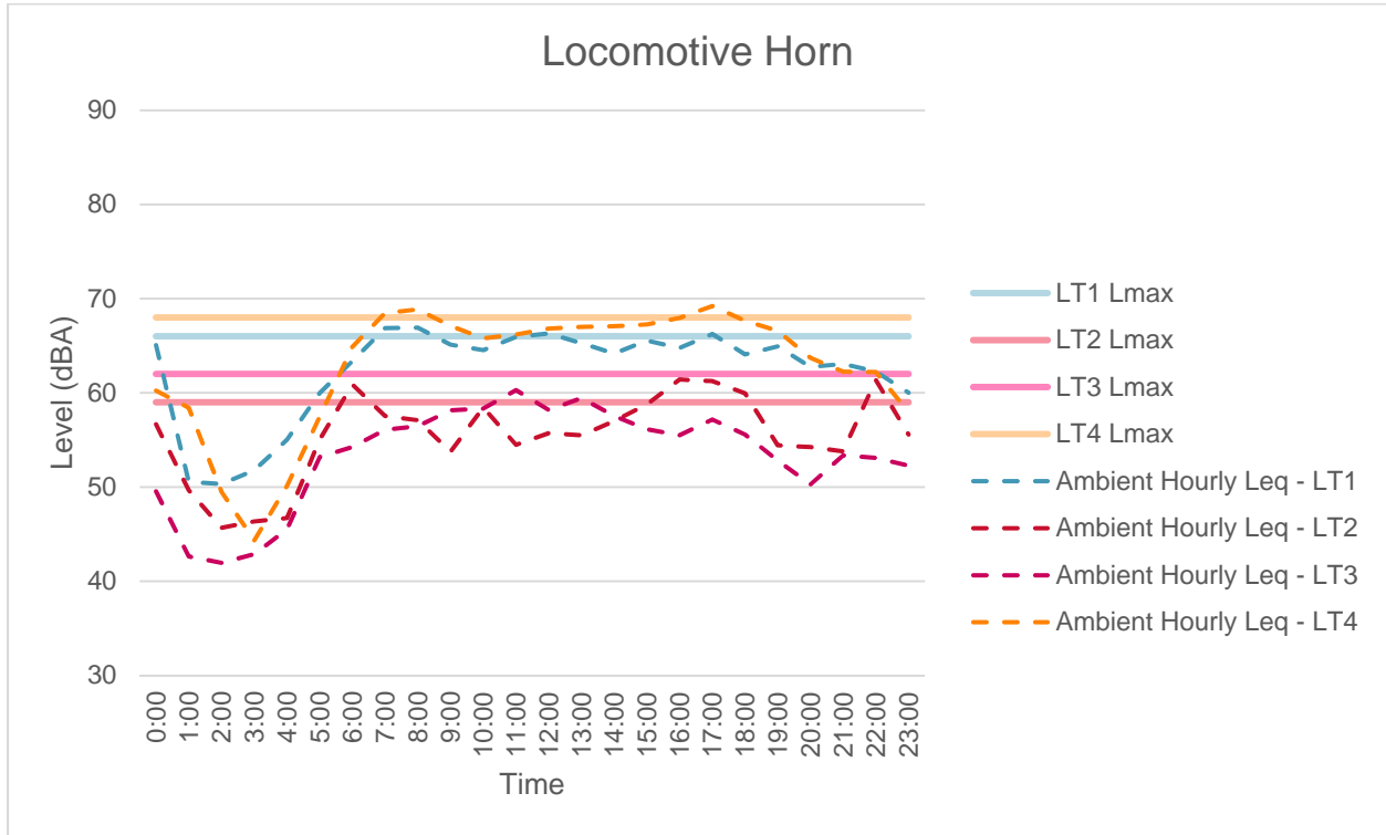
Figure 4-15. Locomotive Horn Lmax vs. Leq at 24-hour Measurement Locations
