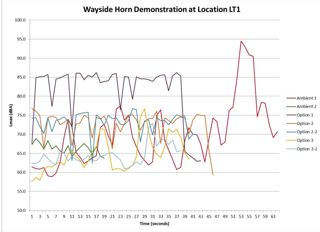
Figure 4-7. Wayside Horn Lmax at LT1
