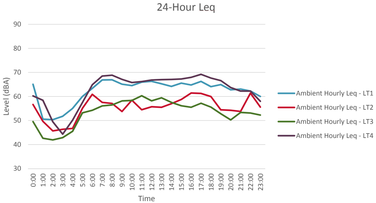
Figure 4-3. Graphical Comparison of Hourly Leq Values
