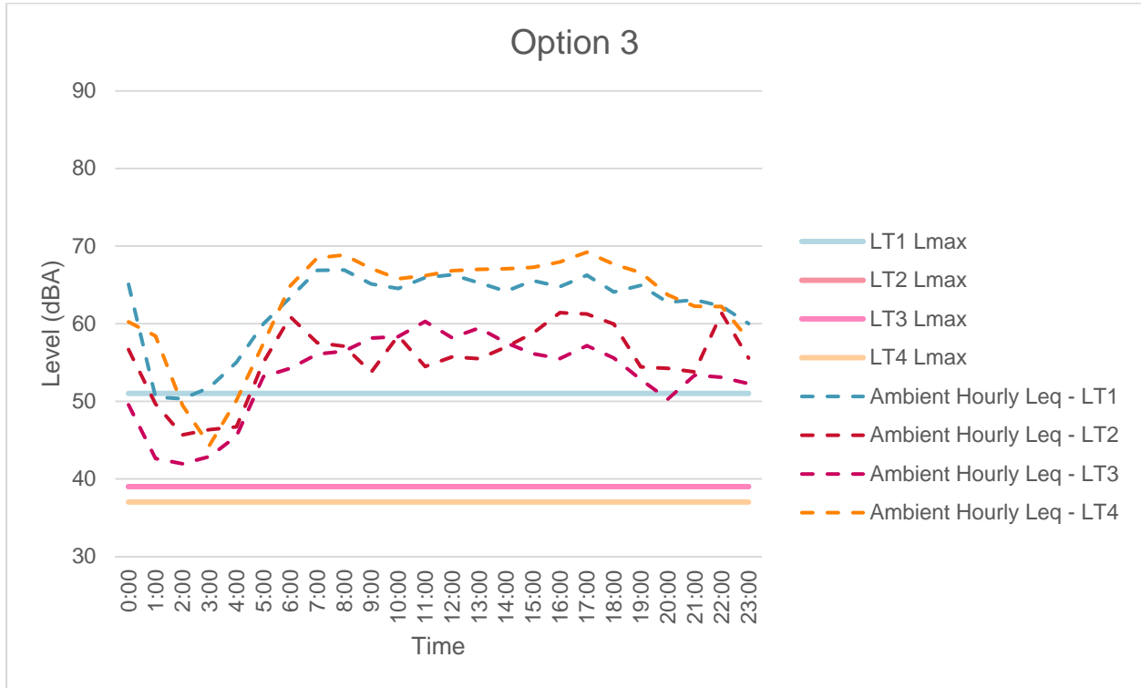
Figure 4-14. Option 3 Lmax vs. Leq at 24-hour Measurement Locations
