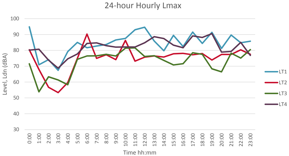
Figure 4-4. Graphical Comparison of Hourly Lmax Values
