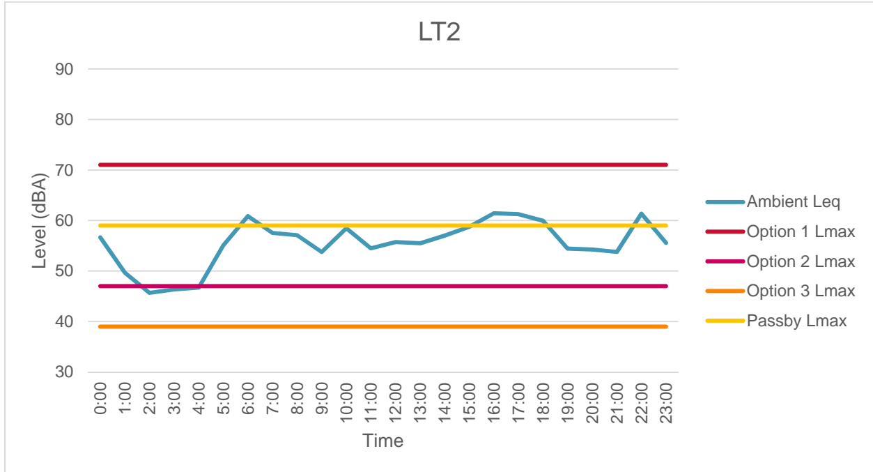
Figure 4-9. Comparison of Wayside Horns Lmax and Ambient Leq at LT2
