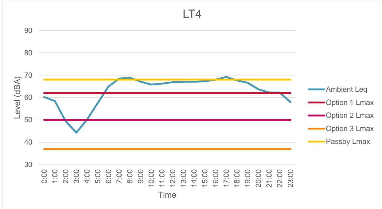
Figure 4-11. Comparison of Wayside Horns Lmax and Ambient Leq at LT4
