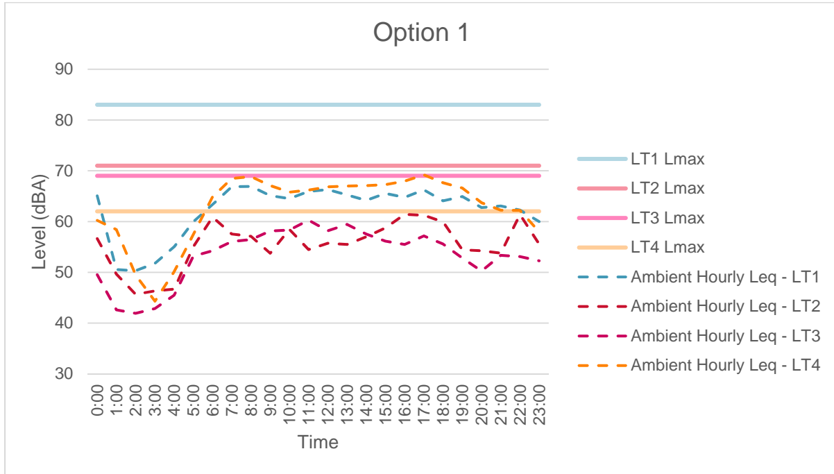
Figure 4-12. Option 1 Lmax vs. Leq at 24-hour Measurement Locations
